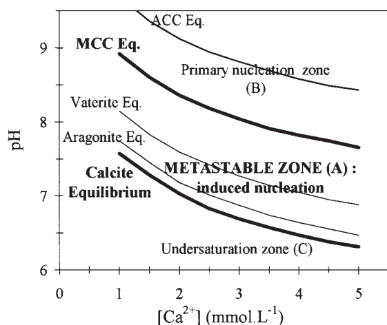
Figure 12. Demarcation of the metastable zone (A) for the "CaCO 3 -CO 2 -H 2 O" system.
