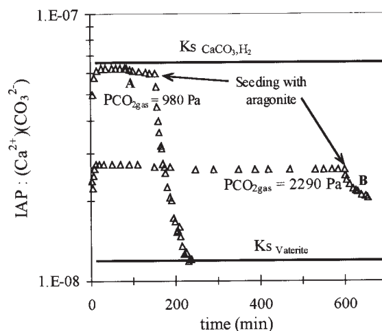
Figure 7. Evolution of the IAP in the metastable zone and precipitation induced with seeding at 30^\circ\text{C} .
